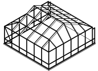
Modified Hip Roof
